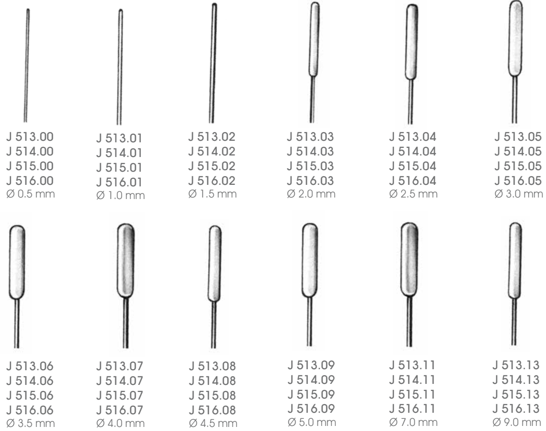
GARRET J 513.00 - J 513.13 14 cm J 514.00 - J 514.13 19 cm J 515.00 - J 515.13 21 cm J 516.00 - J 516.13 35 cm Bükülebilir/Malleable
